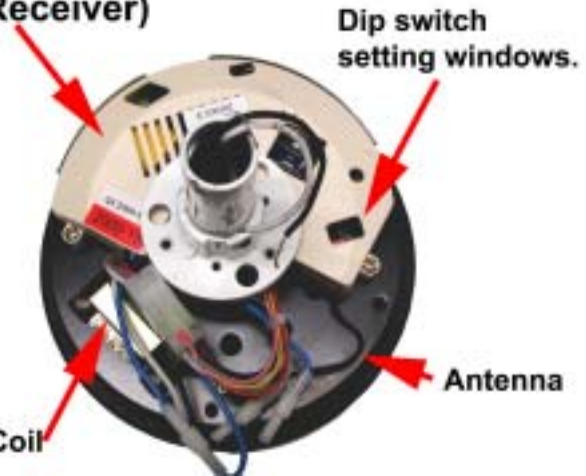
Electronics PC Board (Receiver)
