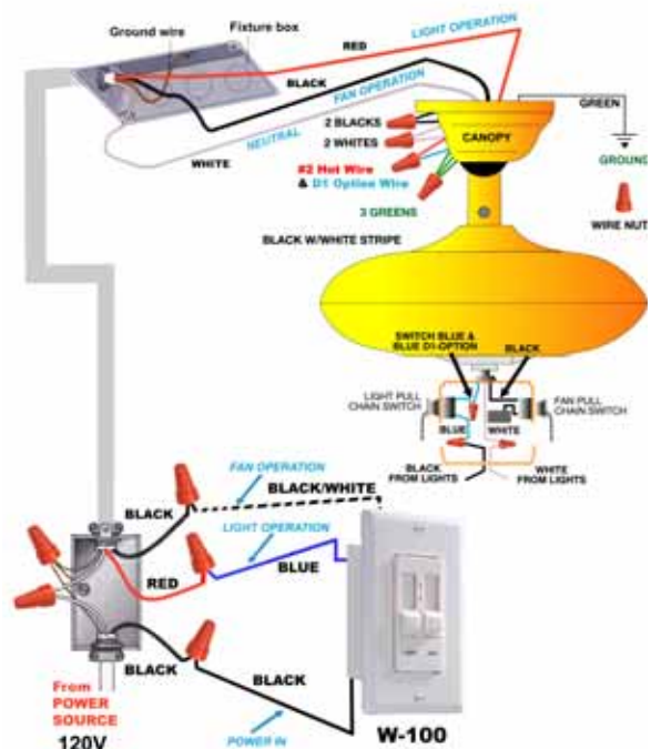
W-100 DUAL SLIDE WALL CONTROL WIRING DIAGRAM - (With-Out Ground Wire)
